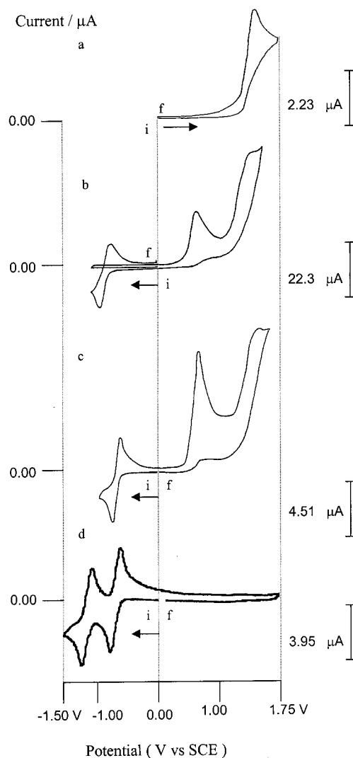
Figure 1. (a) Cyclic voltammetry of n\text{BuNH}_2 (10.0 mM) in DMF + 0.1 M n\text{Bu}_4\text{NBF}_4 at 10 °C; scan rate 0.5 Vs -1 , glassy carbon disc electrode (0.05 mm diameter); the scan is in the potential range: 0.00/1.75/0.00 V; (b) cyclic voltammetry of a mixture of 1 (20.0 mM) and n\text{BuNH}_2 in the presence of t\text{BuOK} (1:5:2) in DMF + 0.1 M n\text{Bu}_4\text{NBF}_4 under an inert gas at 10 °C; scan rate 1.0 Vs -1 , glassy carbon disc electrode (0.05 mm diameter); the scan is in the potential range: 0.00/1.75/0.00 V (2 cycles); (c) cyclic voltammetry of a mixture of 1 (20.0 mM) and n\text{BuNH}_2 in the presence of n\text{Bu}_4\text{NF}\cdot 3\text{H}_2\text{O} (1:5:5) in DMF + 0.1 M n\text{Bu}_4\text{NBF}_4 under an inert gas at 10 °C; scan rate 1.0 Vs -1 , glassy carbon disc electrode (0.05 mm diameter); the scan is in the potential range: 0.00/1.75/0.00 V; (d) cyclic voltammetry of 1 (6.0 mM) in DMF + 0.1 M n\text{Bu}_4\text{NBF}_4 at 13 °C; scan rate 1.0 Vs -1 , glassy carbon disc electrode (0.05 mm diameter); the scan is in the potential range: 0.00/1.75/0.00 V
